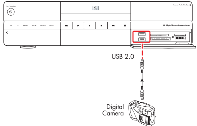
Digital still camera connection (front panel)
